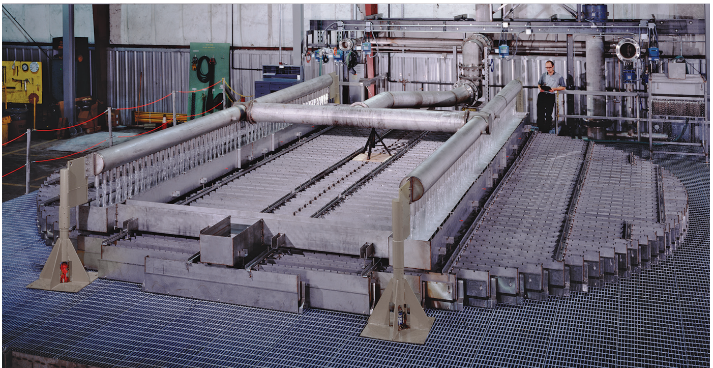
KOCH-GLITSCH'S COMMERCIAL-SCALE DISTRIBUTOR TEST FACILITY, WICHITA, KANSAS, USA
