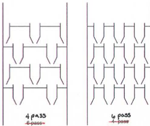
Figure 1. Schematic of original and replacement trays.
