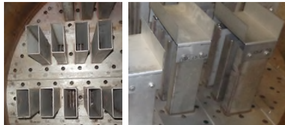
Figure 4. The deck distributor and redistributor (post-revamp).
