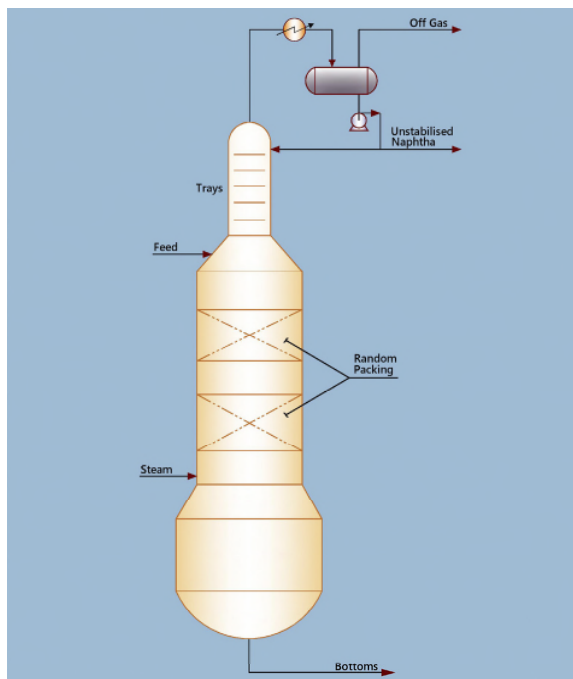
Figure 1. A hydrocracker/DHT stripper.
