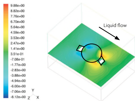
Figure 2. Liquid push towards the outlet weir is created by vapour.
