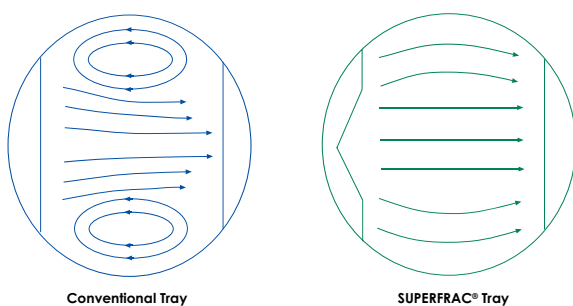
Figure 3. A comparison of the liquid flow pattern of trays.
