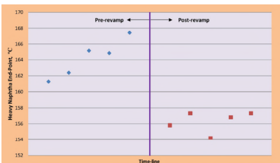
Figure 6. Combined HCU/DHT stripper heavy naphtha endpoint.
