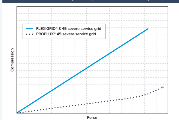
FIGURE 3 Strength Comparison of Grid Packings
