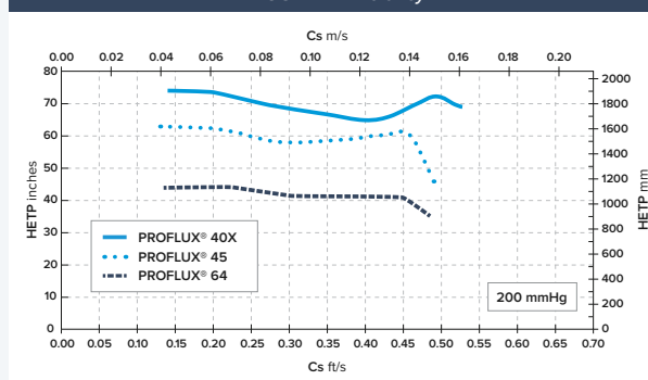
FIGURE 2 Efficiency
