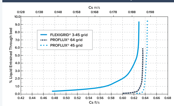
FIGURE 1 De-entrainment Efficiency
