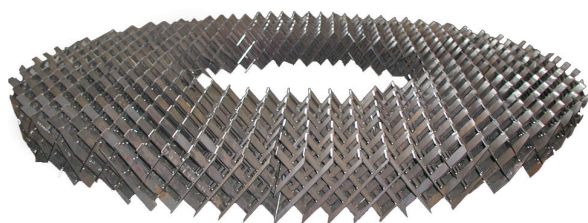
ANNULAR KFBE PACKING FOR INSTALLATION AROUND THE REACTION RISER
