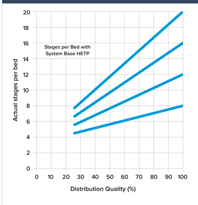
THE EFFECT OF LIQUID DISTRIBUTION QUALITY ON TOWER PERFORMANCE
