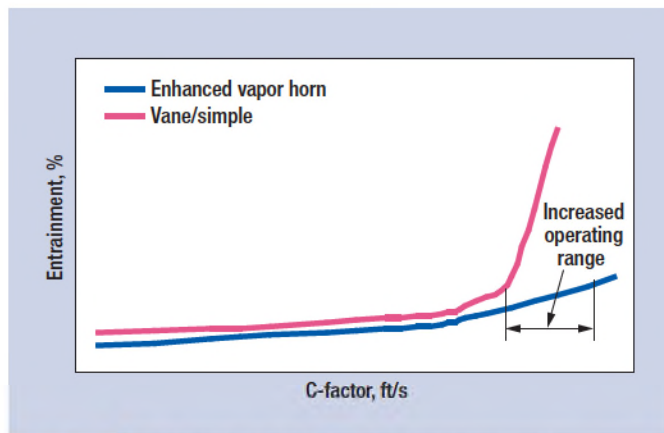
FIG. 4 Inlet feed device relative performance comparison.
