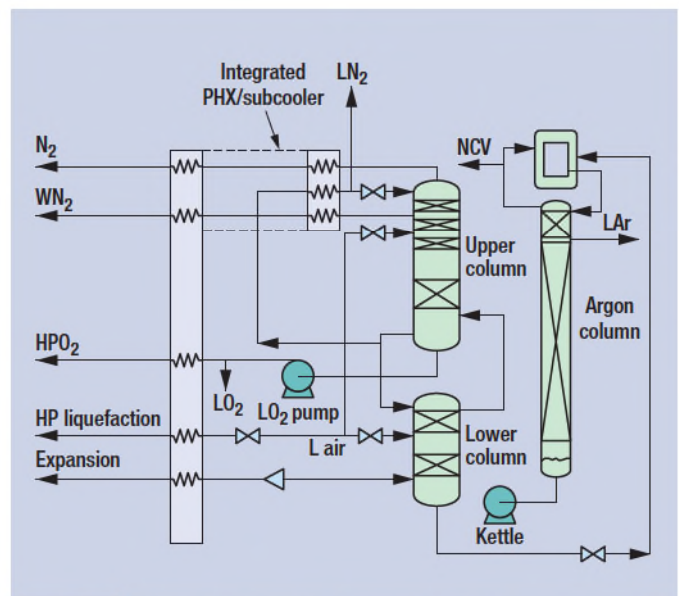
FIG. 6 Schematic of a typical air separation unit.
