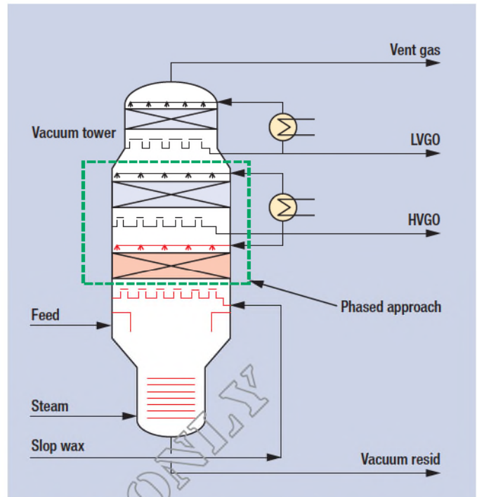
FIG. 5 Vacuum column design using phased approach.
